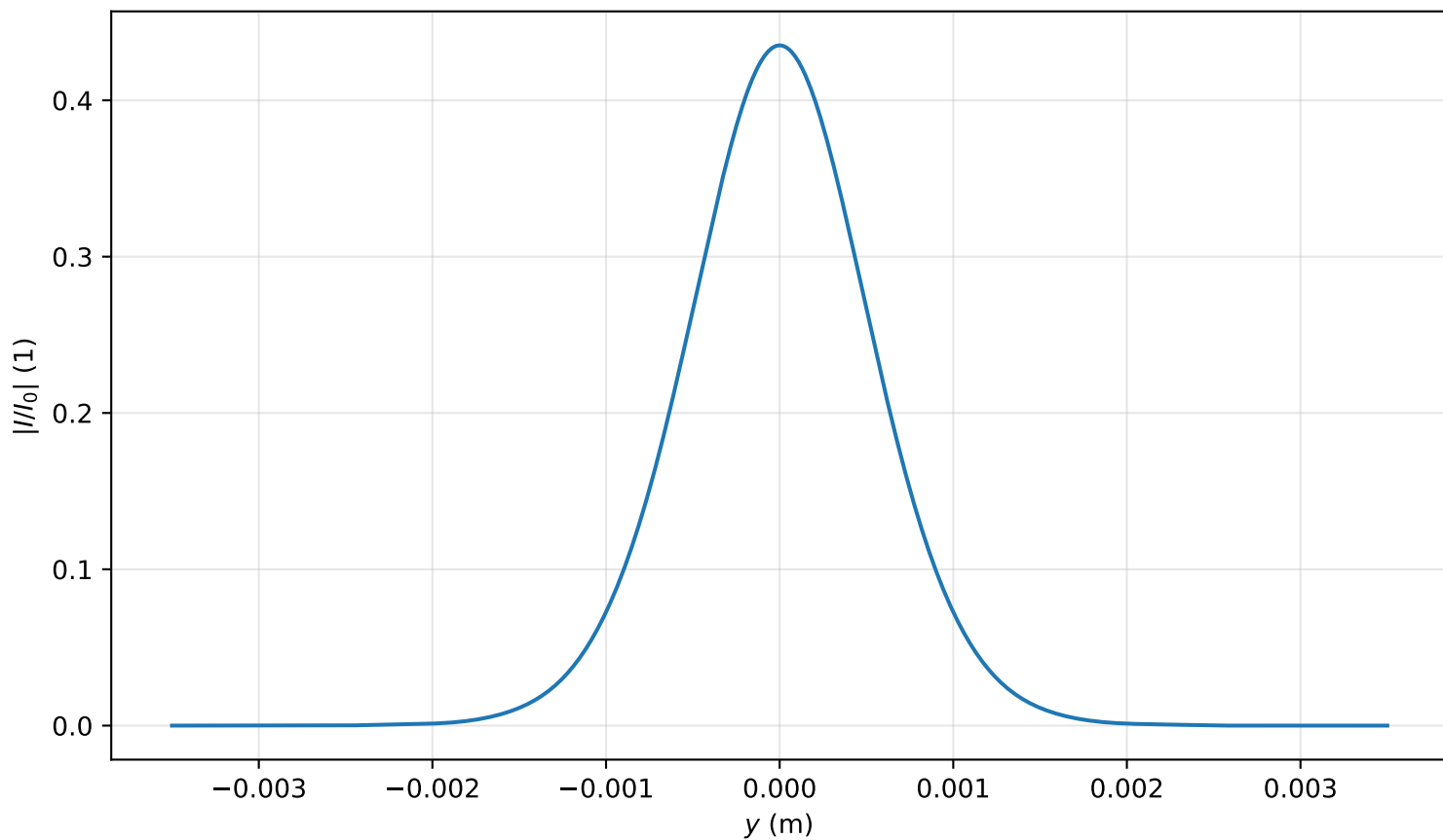
Intensity profile I(x=0, y, z=3.264)/I_0 , P_{in}=0.4P_{cr} , artificial time
